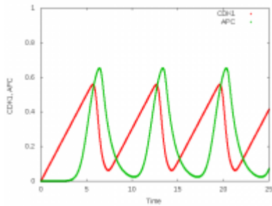
Time plots of ODE model of Xenopus embryonic cell cycle, modeled with delay differential equations
